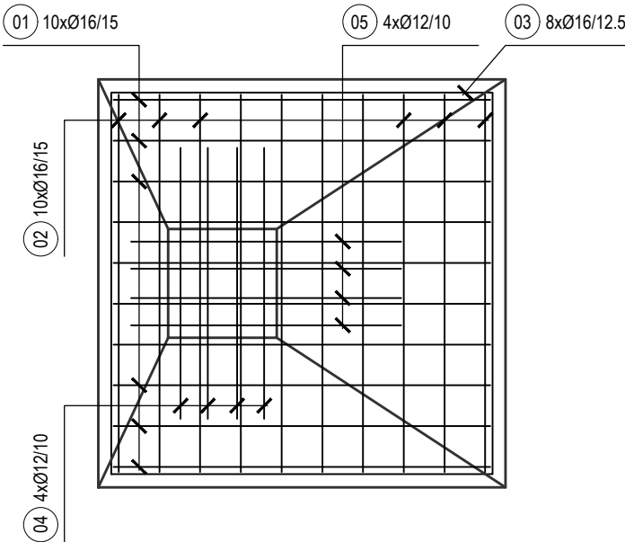
ISKAZ ARMATURE MJ 1:50
