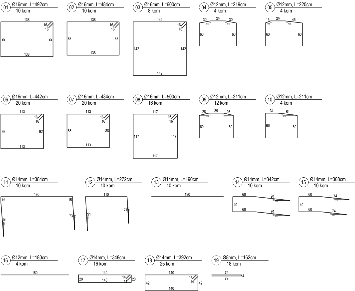
ISKAZ ARMATURE MJ 1:50
